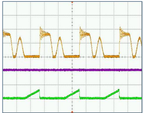
AC100V Bottom skip
