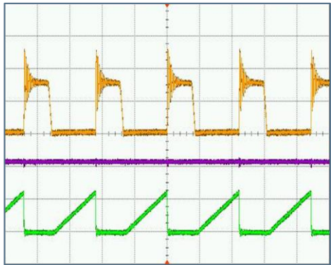
AC100V Maximum load
